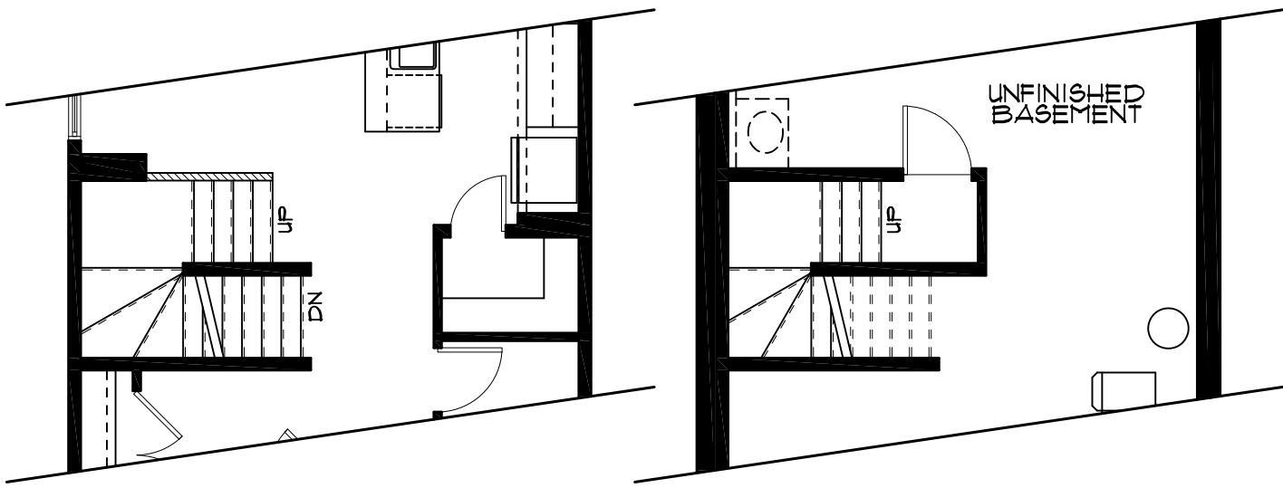
DEVELOPED STAIR OPTION
